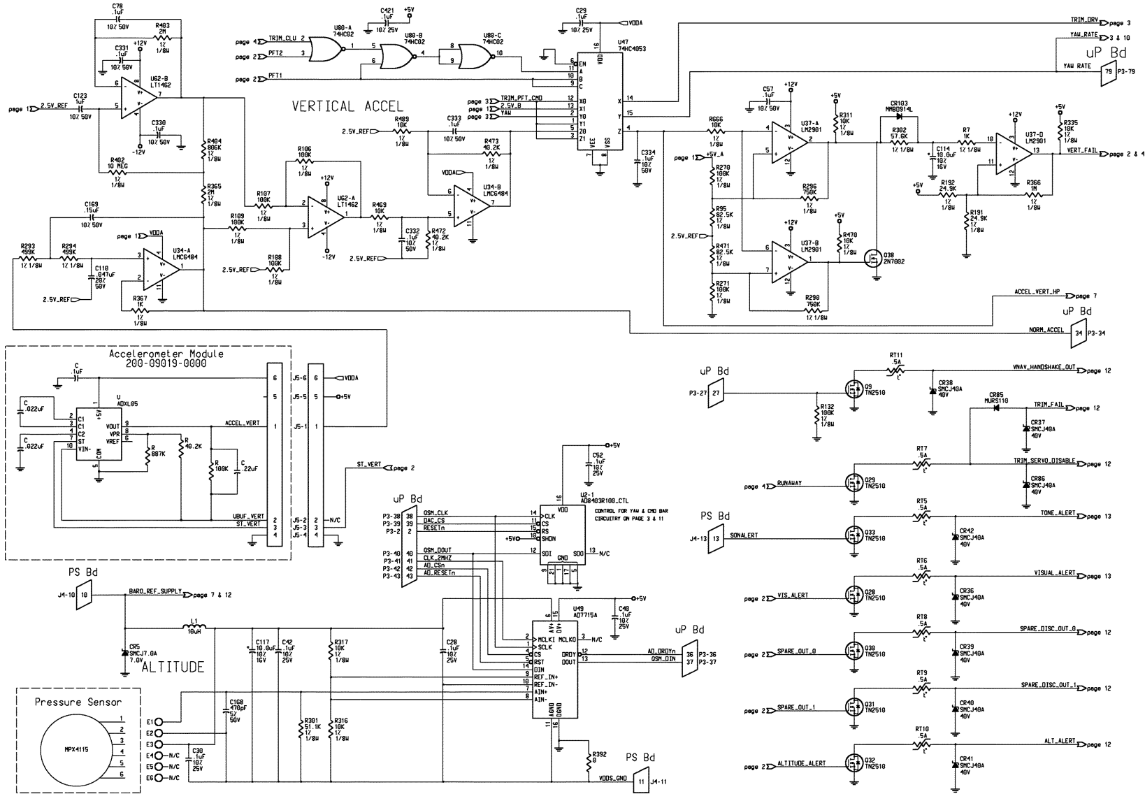
FIGURE 6-9 I/O BOARD SCHEMATIC (Sheet 6 of 13)
