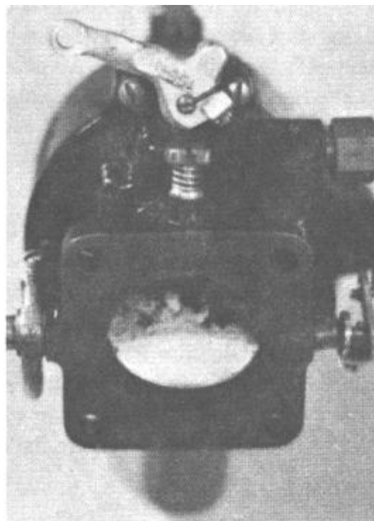
CARBURETOR ICE
